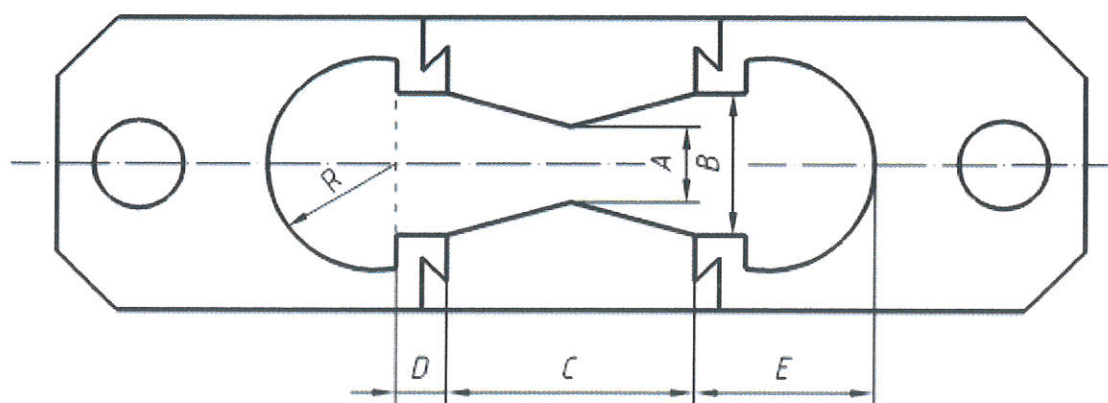
Figure 1 : Moule type
